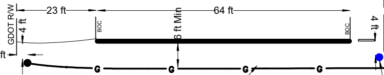
Profile for Bore at New St & Kirby Ave Crossing
