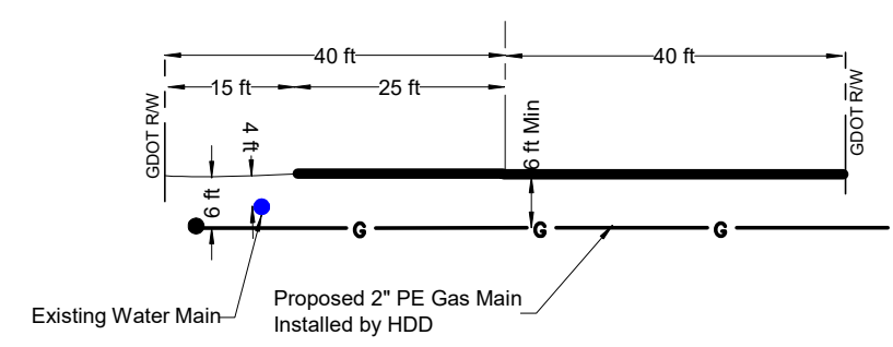
Profile for Bore at Lowe Rd Crossing
